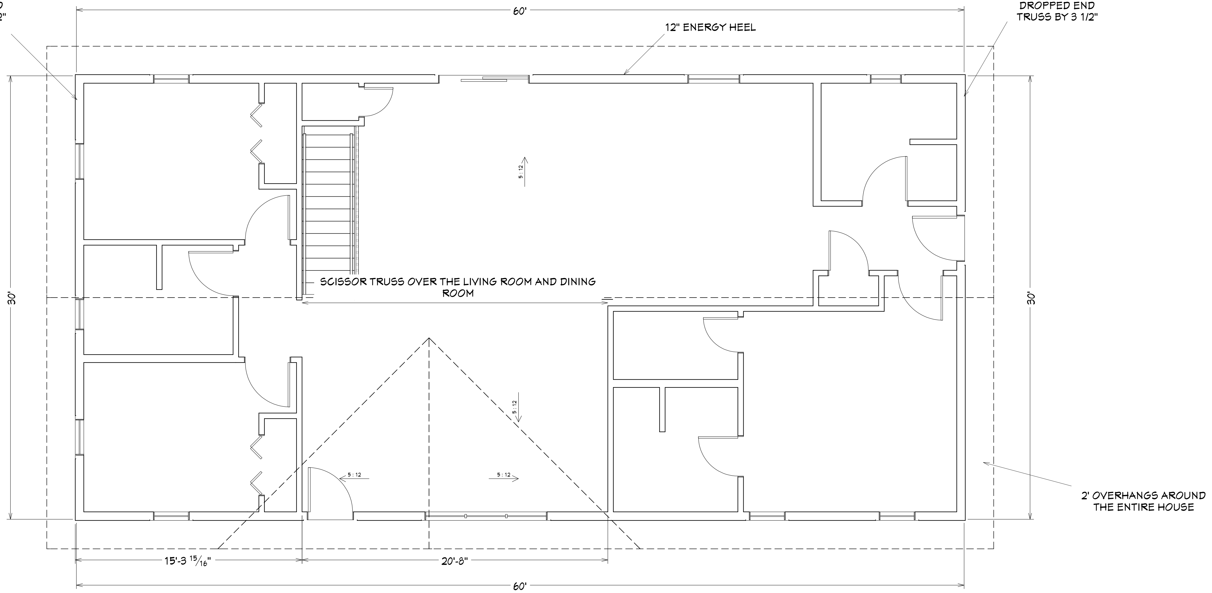
ROOF PLAN VIEW 5/16 IN = 1 FT
