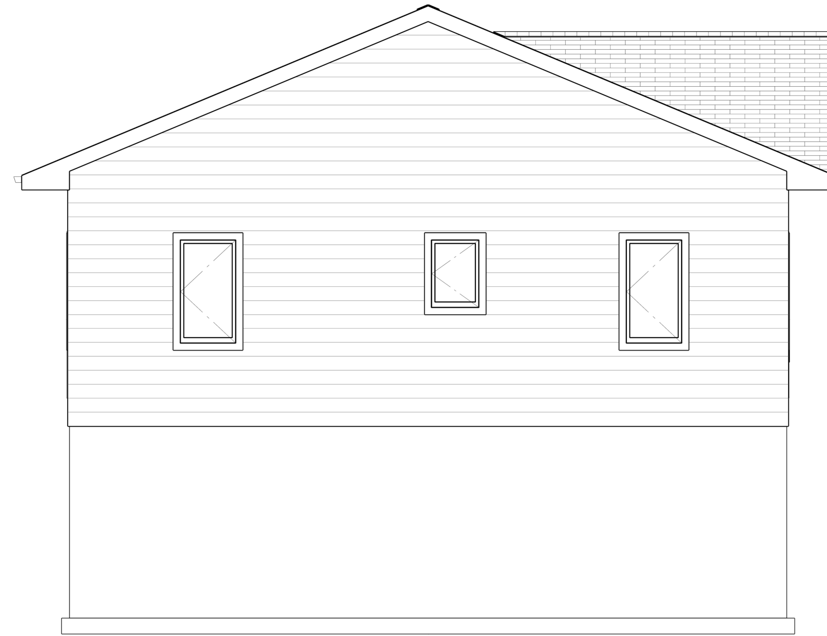
E4 ELEVATION 4 1/4 IN = 1 FT
